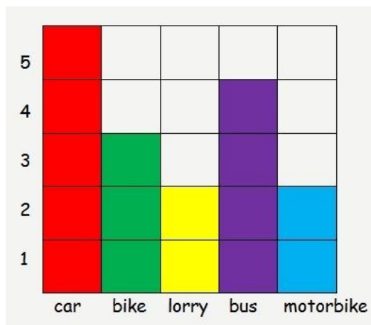
Block Graph
