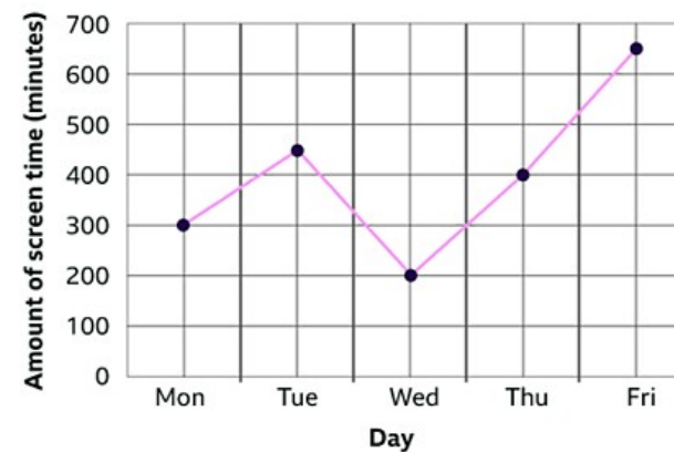
Line Graph
